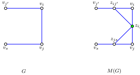
Figure 4. A part of the middle graph of G .
