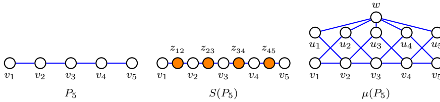
Figure 1. A path, its subdivision and Mycielskian
