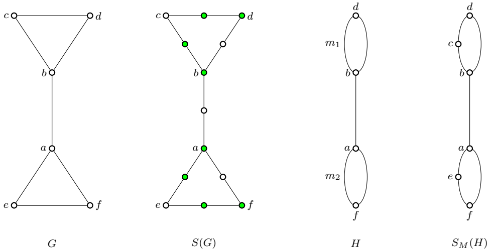
Figure 2. Graphs corresponding to Example 1.
