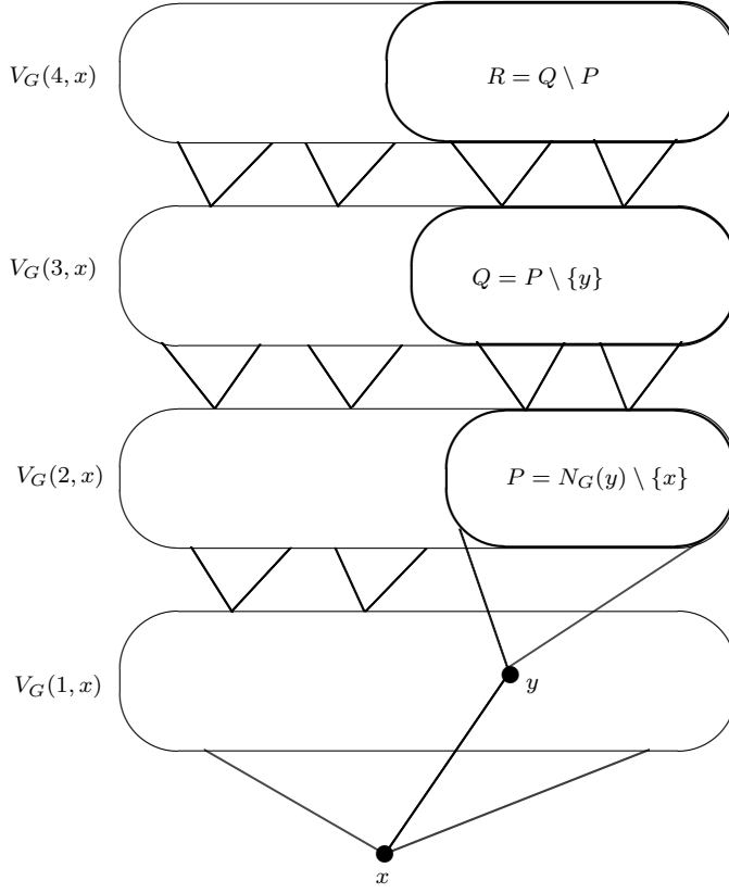
Figure 2. The sets P, Q, R.
