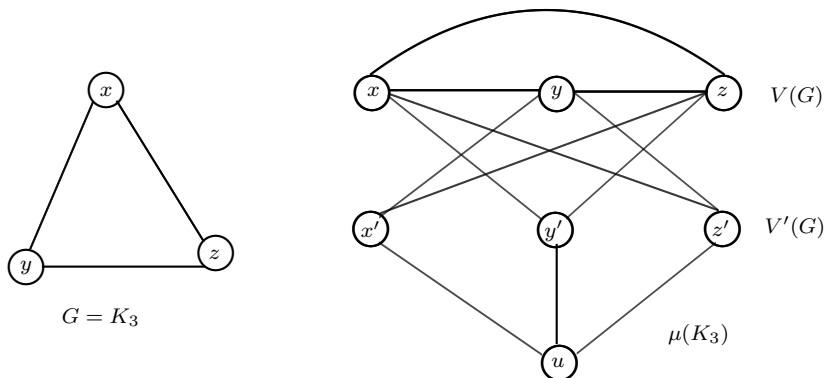
Figure 1. Mycielskian of K_3
