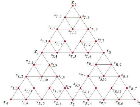
Figure 5. Labeling of Sierpiński triangle graph S_4
