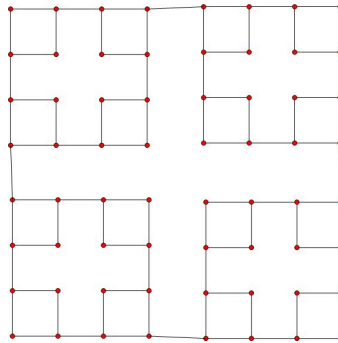
Figure 1. Generalized Sierpiński graph S(C_4, 3)
