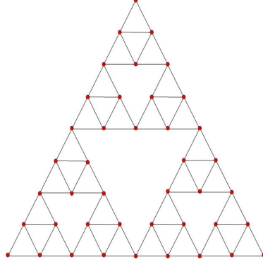
Figure 3. Sierpiński triangle graph S_4
