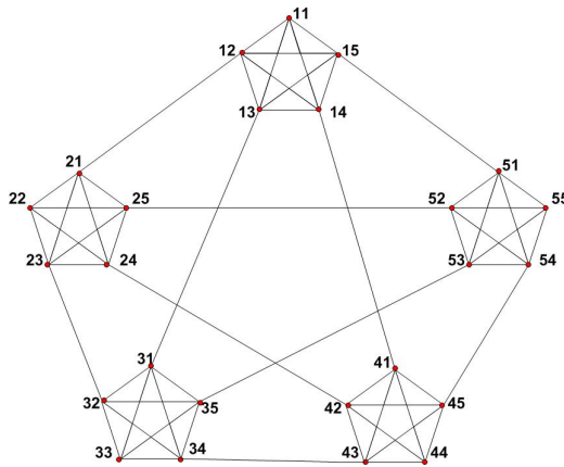
Figure 2. Sierpiński graph S(K_5, 2)
