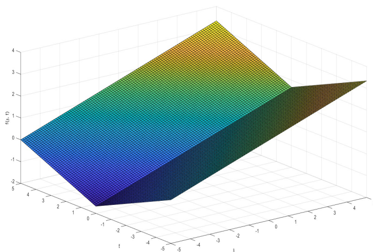
Figure 1. The plot of the objective function \Gamma(\bar{z}, \bar{t}) = \frac{1}{3}\bar{z} + \frac{1}{3}|\bar{t}| of the (\mathcal{EH}) in Example 1.
