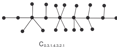
Figure 3. Example of caterpillar tree.
