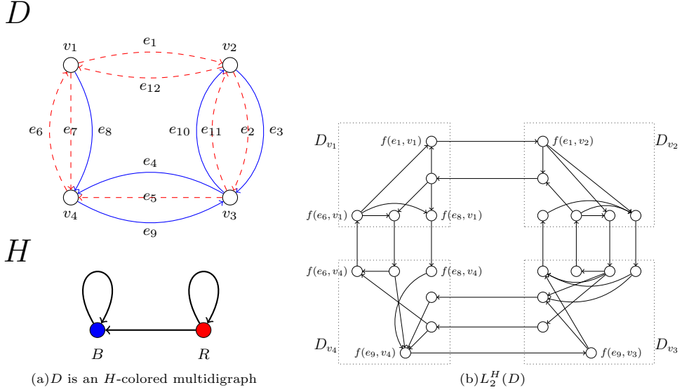
Figure 1. The auxiliary digraph L_2^H(D)
