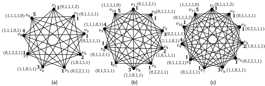
Figure 6. A locating rainbow coloring of (a) \overline{C}_9 , (b) \overline{C}_{10} , and (c) \overline{C}_{11} .
