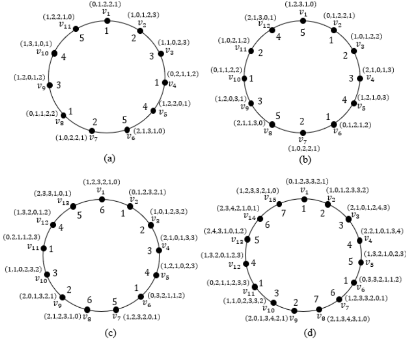
Figure 3. A locating rainbow coloring of (a) C_{11} , (b) C_{12} , (c) C_{13} , and C_{15} .
