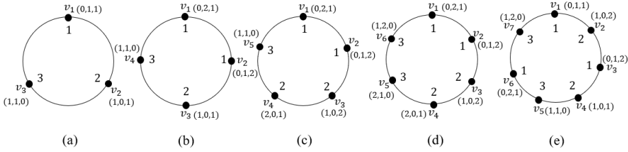
Figure 1. Locating rainbow 3-colorings of (a) C_3 , (b) C_4 , (c) C_5 , (d) C_6 , and (e) C_7 .
