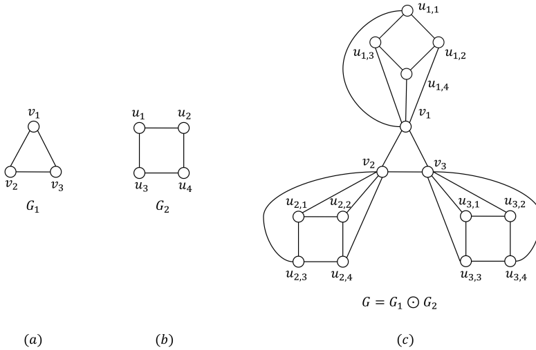
Figure 2. the graph G_1 (a), the graph G_2 (b) and the corona graph G = G_1 \odot G_2 (c).
