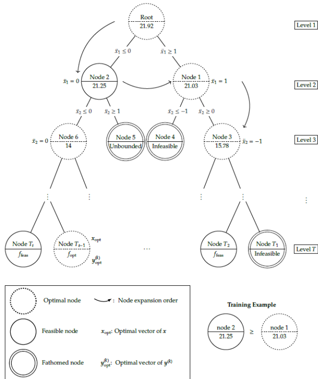
Figure 3. A schematic creation of a branch-and-bound tree while solving underlying subproblems ( K = 5 ).
