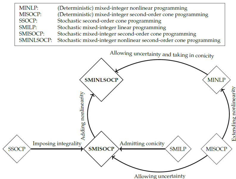
Figure 1. Conceptual relationships between SMISOCP and SMINLSOCP problems and other relevant optimization problems.
