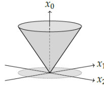
Figure 2. The 3rd-dimensional second-order cone \mathcal{E}_+^3 \triangleq \{(x_0; x_1; x_2) \in \mathcal{E}^3 : x_0 \geq \sqrt{x_1^2 + x_2^2}\} .
