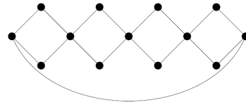
Figure 2. Planar embedding of \mu_3(P_3) .
