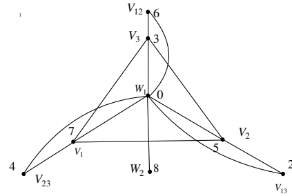
Figure 4. \Gamma'((\mathbb{Z}_2)^3)
