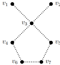
Figure 2. A signed graph \Sigma with \text{sbdim}(\Sigma) = 3
