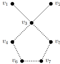
Figure 3. The 1-switched signed graph \Sigma^n with \text{sbdim}(\Sigma^n) = 2
