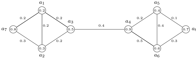
Figure 1. A graph G = (\sigma, \mu) with ssd(G) = 0.9
