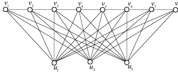
Figure 2. The graph P_8 + \overline{K}_3 .
